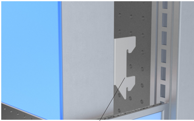
Laser cut bracket to engage upright
